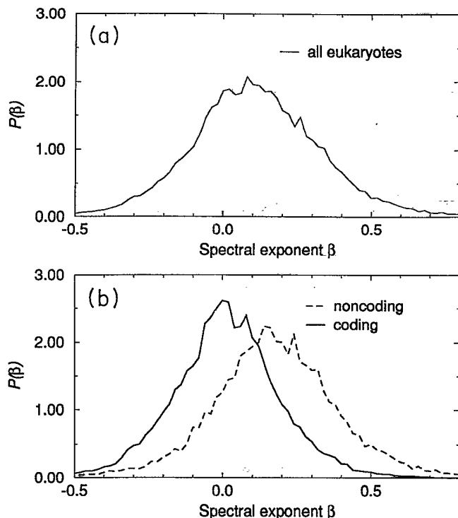
FIG. 2. Histograms of the values of \beta obtained for all coding and noncoding eukaryotic sequences > 512 bp of the GenBank by the FFT method. The probability density of finding a value of \beta between \beta and \beta + d\beta is plotted against \beta (purine-pyrimidine rule of mapping). (a) Coding and noncoding sequences combined together, (b) coding and noncoding sequences analyzed separately.
